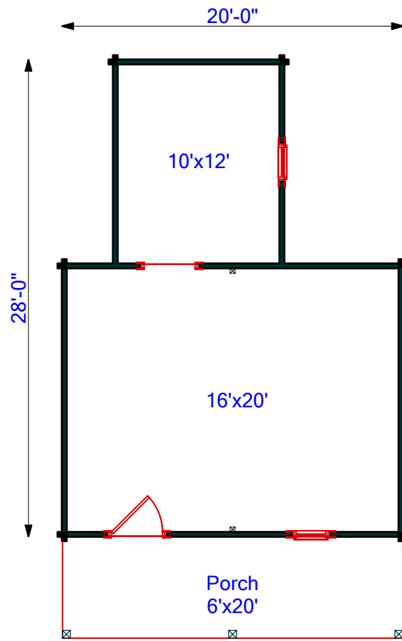
Floor Plan
